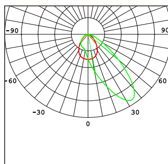
Asymmetrical intense 35° F04001@300W
