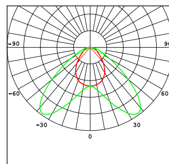
Asymmetrical intense 2Tilt35° F04001@600W
